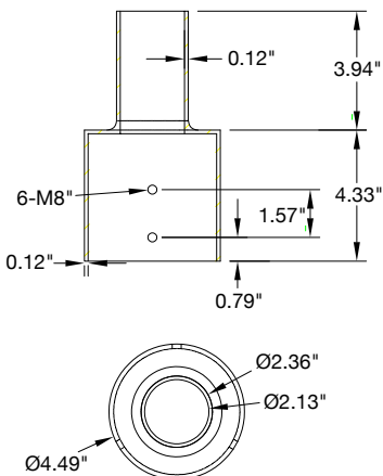
Part #: ETN-RD-4 Description: Tenon: Round 4" Pole Reducer to 2.36" Bracket EPA: 0.4
