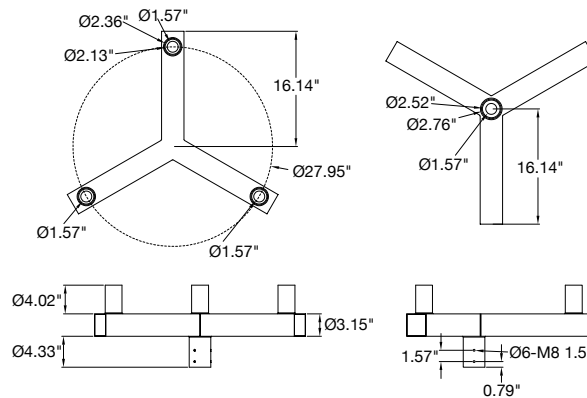
Part #: ETN-BH-SQ-180-3Y Tenon: Square Bullhorn 3-Head Y-Adapter Bracket EPA: 1.9
