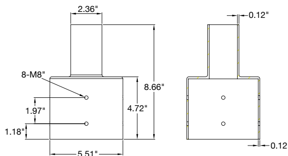
Part #: ETN-RD-5 Tenon: Round 5" Pole Reducer to 2.36" Bracket EPA: 0.45
