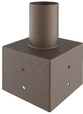
Part #: ETN-SQ-4 Tenon: Square 4" Pole Reducer to 2.36" Bracket EPA: 0.3
