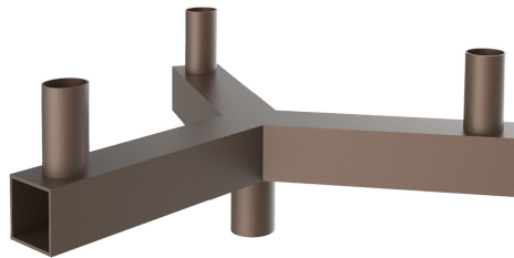
Part #: ETN-BH-SQ-180-3Y Tenon: Square Bullhorn 3-Head Y-Adapter Bracket EPA: 1.9
