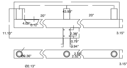
Part #: ETN-BH-SQ-180-3S Tenon: Square Bullhorn 3-Head Adapter Bracket EPA: 1.9
