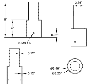
Part #: ETN-RD-3 Tenon: Round 3" Pole Reducer to 2.36" Bracket EPA: 0.4
