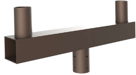
Part #: ETN-BH-SQ-180-2S Tenon: Square Bullhorn 2-Head Adapter Bracket EPA: 1.2
