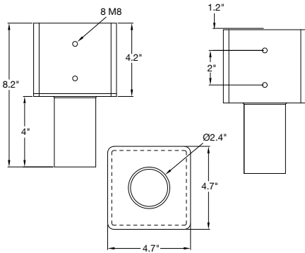
Part #: ETN-SQ-4 Tenon: Square 4" Pole Reducer to 2.36" Bracket EPA: 0.3
