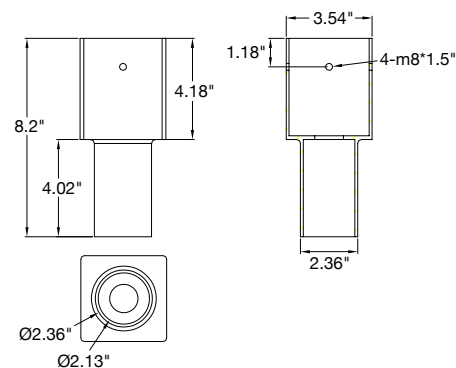
Part #: ETN-SQ-3 Tenon: Square 3" Pole Reducer to 2.36" Bracket EPA: 0.3
