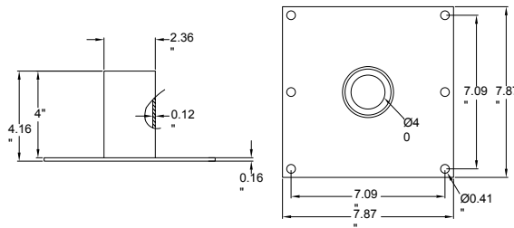
Part #: ETN-WM-7 Tenon: Wall Mount Straight 4" Mounting Bracket Bronze Finish Bracket EPA: 0.2
