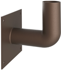
Part #: ETN-WM-90-7 Tenon: Wall Mount 90 Degree Arm 7" Mounting Bracket Bronze Finish Bracket EPA: 0.3
