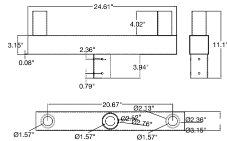
Part #: ETN-BH-SQ-180-2S Tenon: Square Bullhorn 2-Head Adapter Bracket EPA: 1.2
