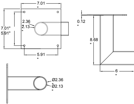
Part #: ETN-WM-90-7 Tenon: Wall Mount 90 Degree Arm 7" Mounting Bracket Bronze Finish Bracket EPA: 0.3
