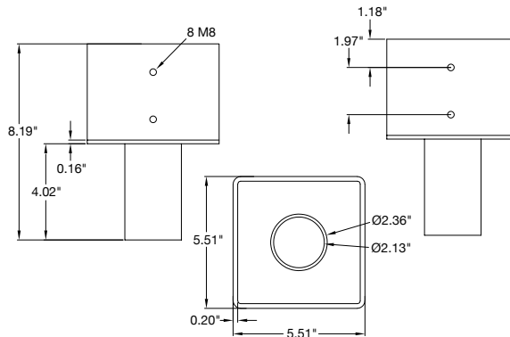
Part #: ETN-SQ-5 Tenon: Square 5" Pole Reducer to 2.36" Bracket EPA: 0.35
