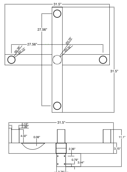
Part #: ETN-BH-SQ-90-4X Tenon: Square Bullhorn 4-Head X-Adapter Bracket EPA: 2
