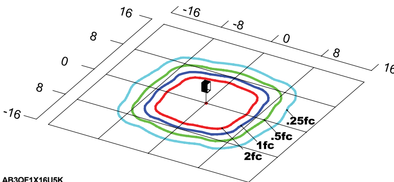
AB3QF1X16U5K Type V Grid in feet, Mounting Height = 3.5 ft.
