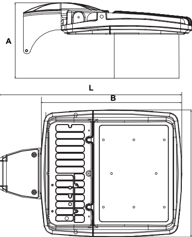
Length with Mount (L)
