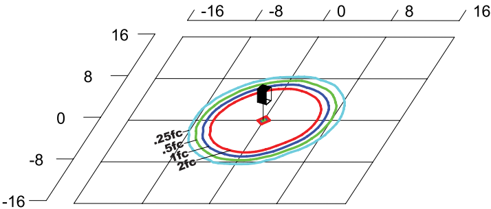
ABORLQF1X15U5K Type V Grid in feet, Mounting Height = 3.5 ft.
