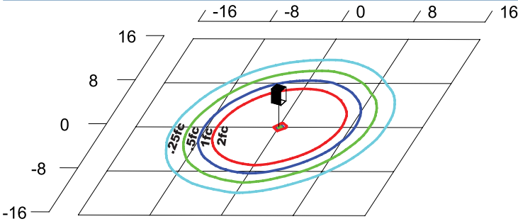
ABOGQF1X15U5K Type V Grid in feet, Mounting Height = 3.5 ft.
