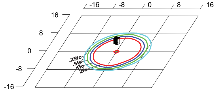
ABOGRLQF1X15U5K Type V Grid in feet, Mounting Height = 3.5 ft.
