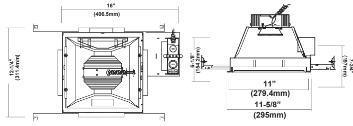
Ceiling Cut-out : 11-1/4" x 11-1/4"
